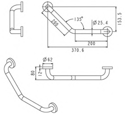
Grab Bar 135° OD 25 mm Size 200×200 mm (Left/Right)
