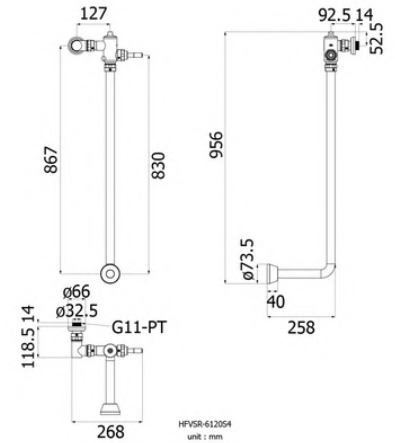
HFVSR-6120S4 unit : mm
