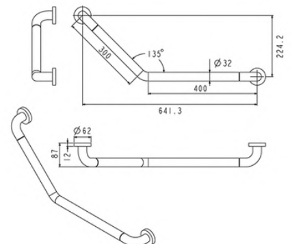
Grab Bar 135° OD 32 mm. Size 300×400 mm. (Right)
