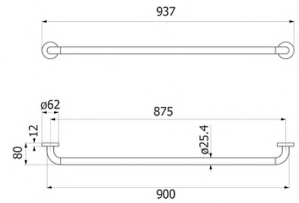
FBVHC-TS790F unit : mm
