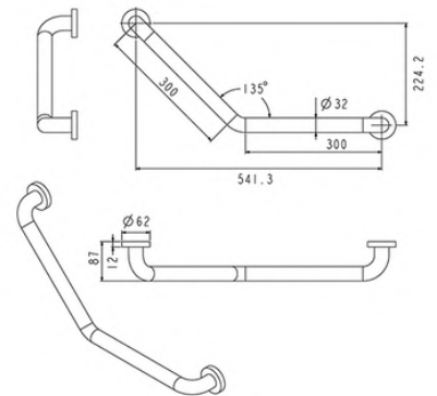
Grab Bar 135° OD 32 mm Size 300×300 mm (Left/Right)
