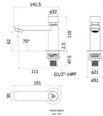
Automatic Self-Closing Basin Faucet T5 Model
