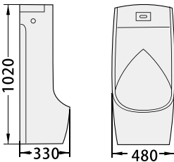
JHU-210 Induction Standing Urinal Size: 480x330x1020mm S-trap Top flushing installation
