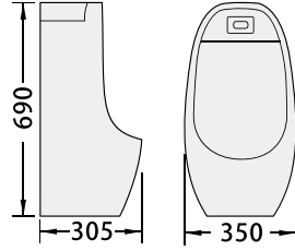
JHU-216 Induction Wall-hung UrinalSize: 350x305x690mm S-trap or P-trap Top flushing installation
