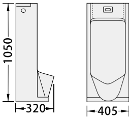
JHU-214 Induction Standing Urinal Size: 405x320x1050mm S-trap Top flushing installation
