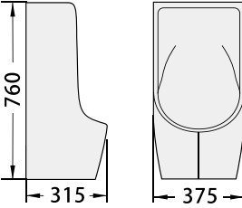
JHU-834 Wall-hung Urinal Size: 375x315x760mm S-trap or P-trap Top flushing installation
